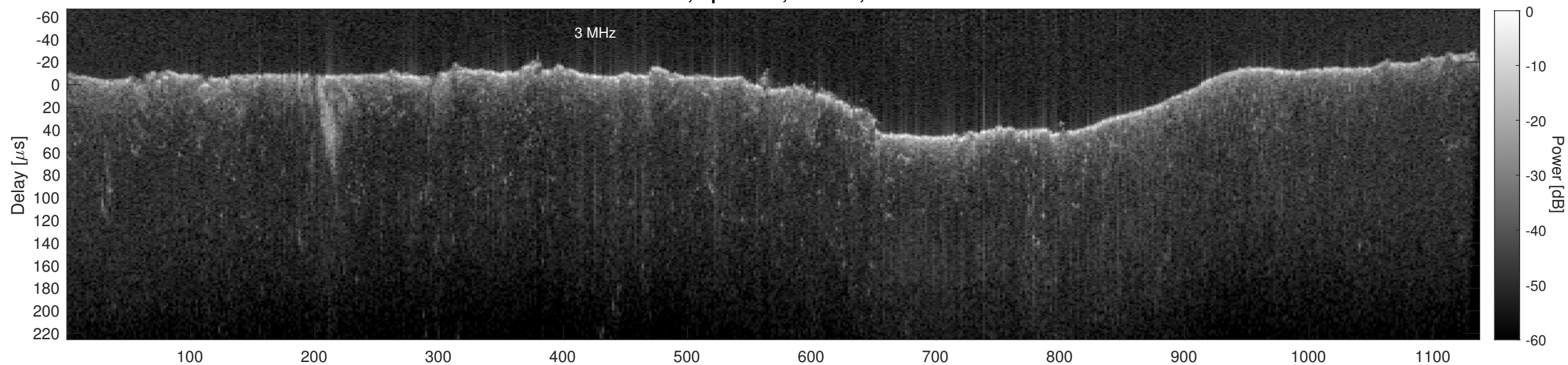
Orbit 21685, Cluttergram
