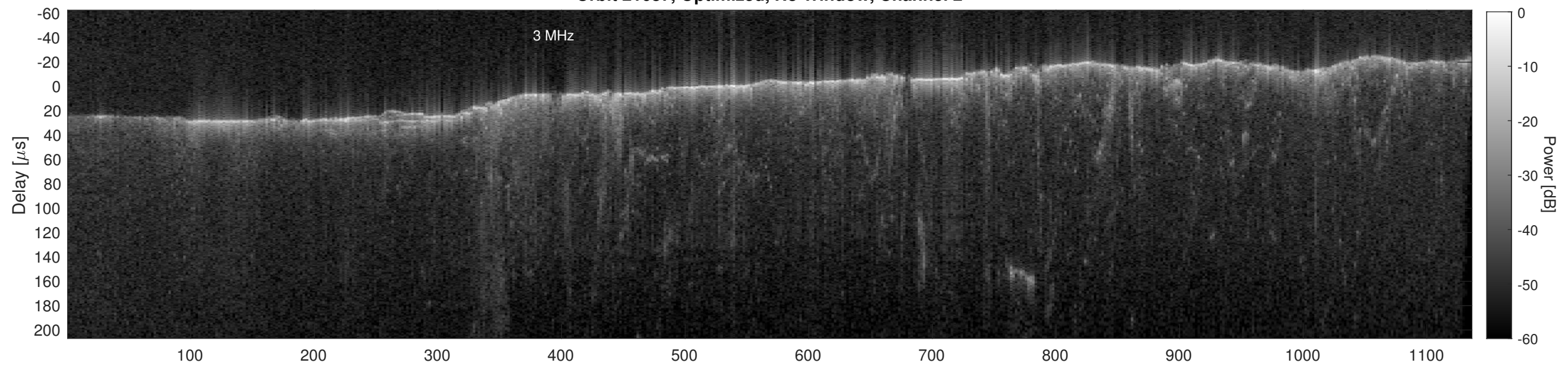
Orbit 21687, Cluttergram
