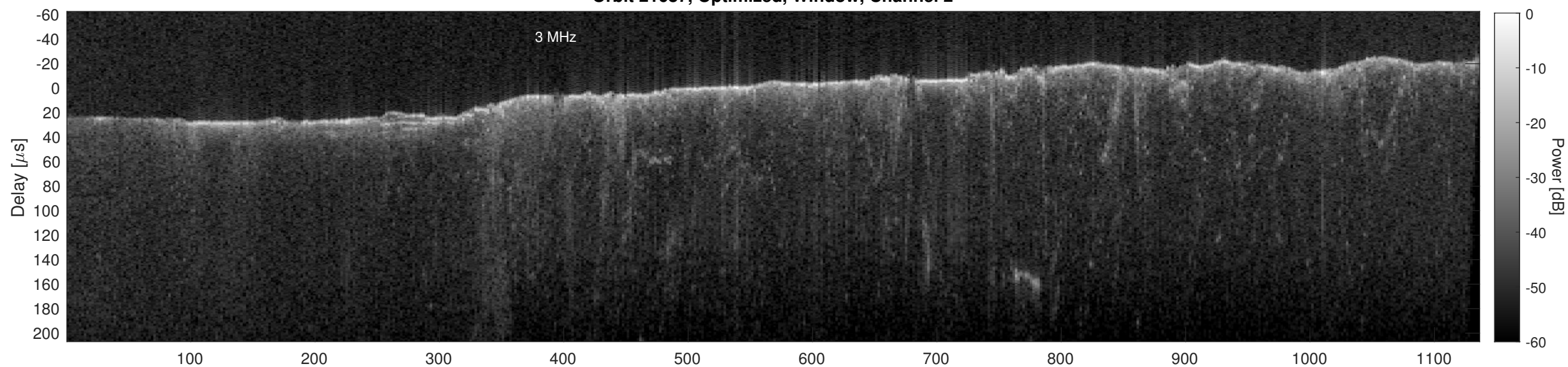
Orbit 21687, Cluttergram
