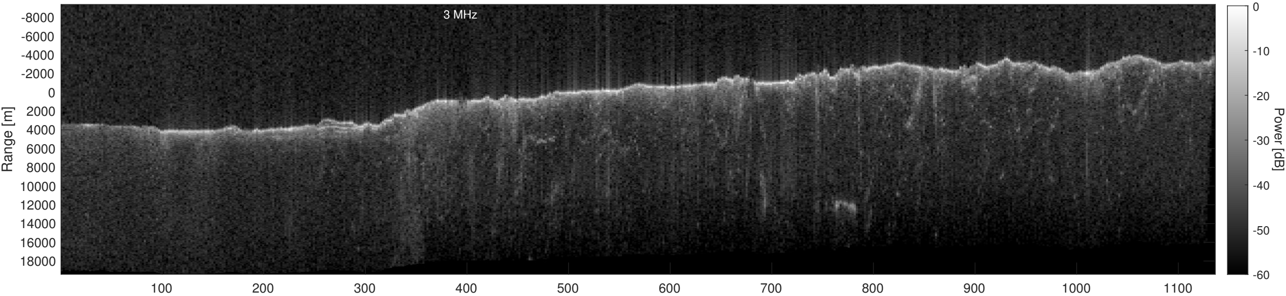
Orbit 21687, Depth-Corrected Cluttergram
