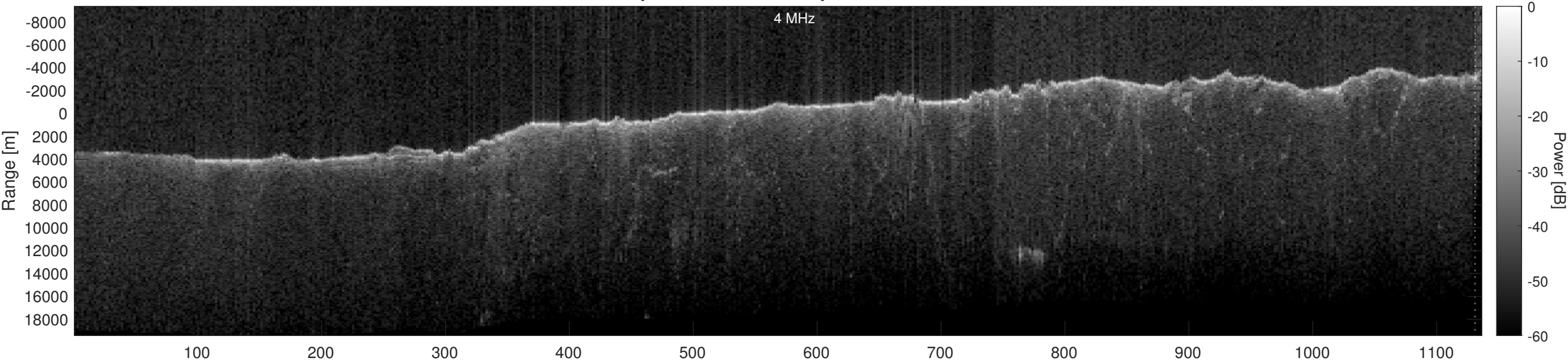
Orbit 21687, Optimized, Window, Depth-Corrected, Channel 2
