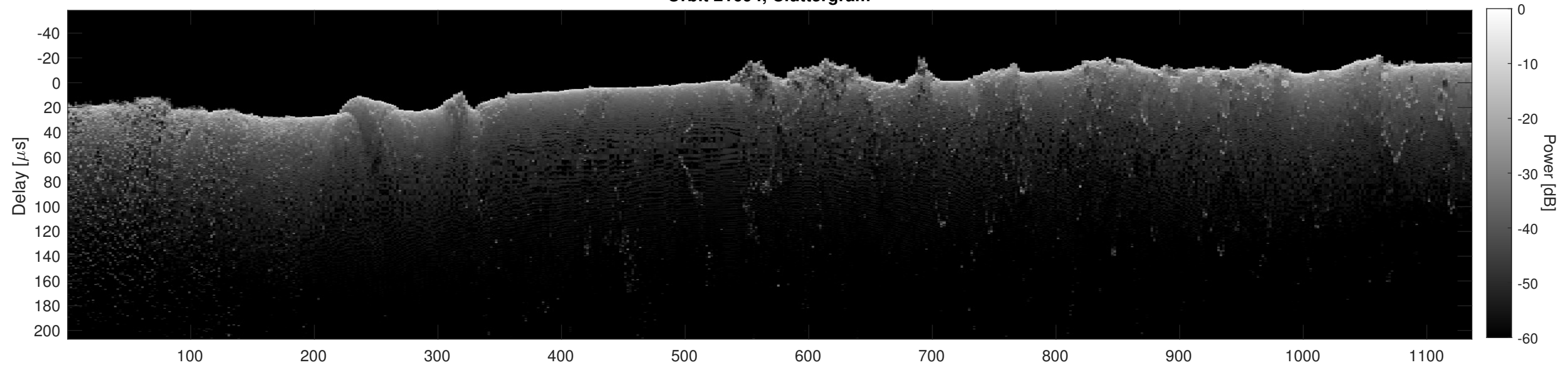
Orbit 21694, Cluttergram
