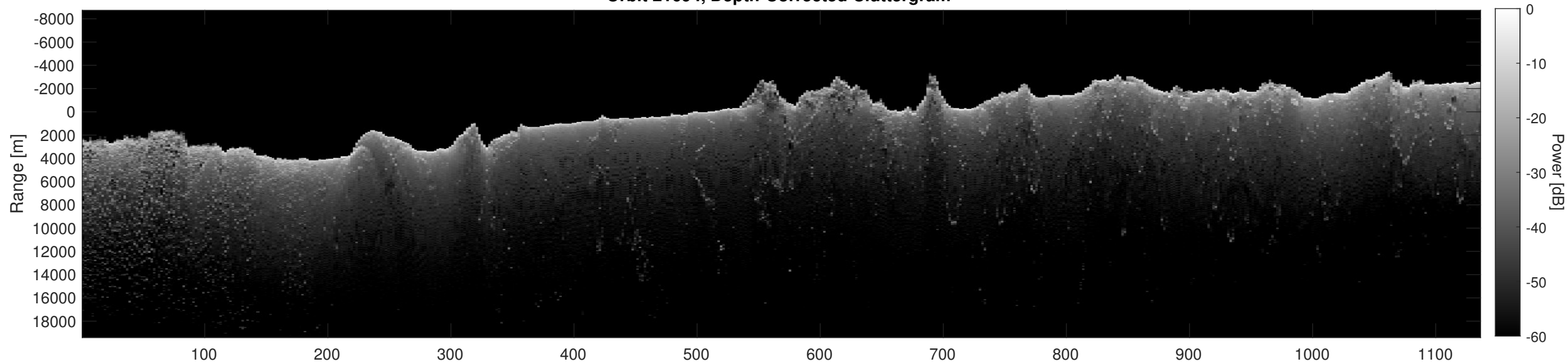
Orbit 21694, Depth-Corrected Cluttergram
