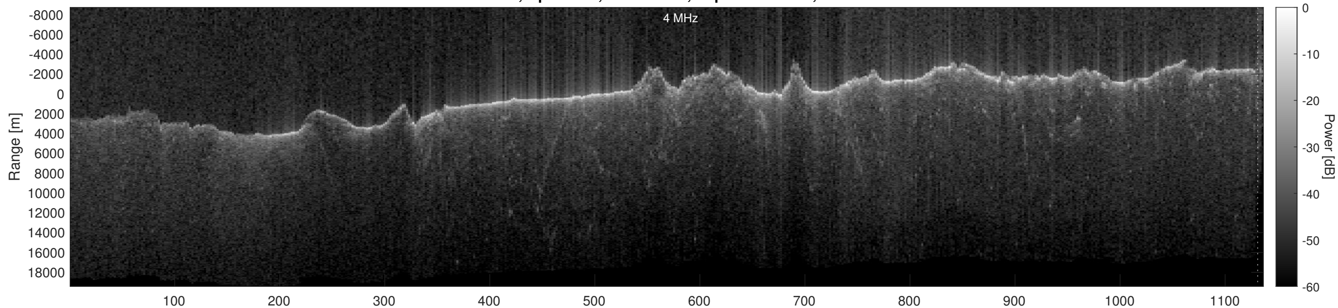
Orbit 21694, Optimized, No Window, Depth-Corrected, Channel 2
