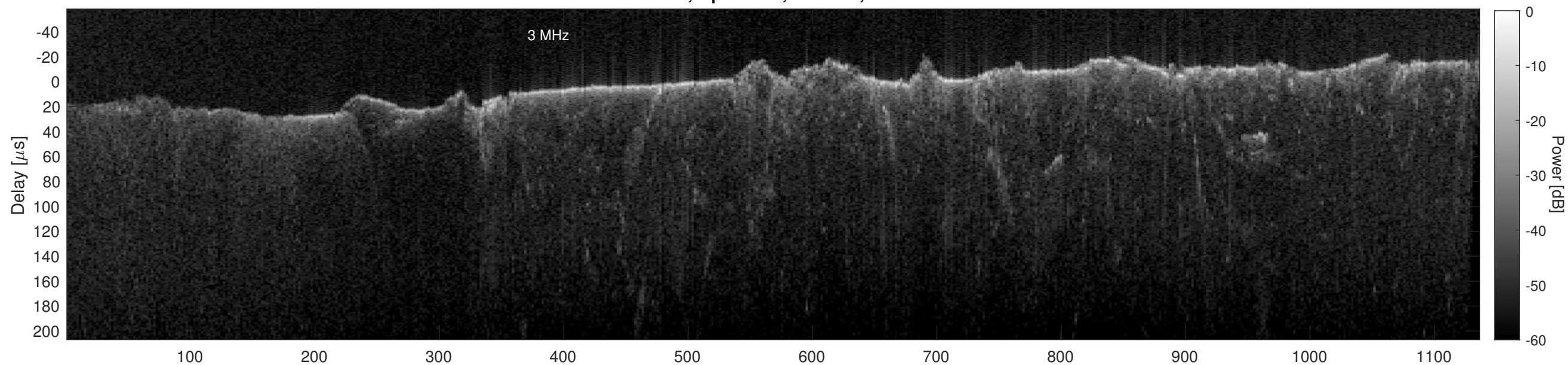
Orbit 21694, Cluttergram
