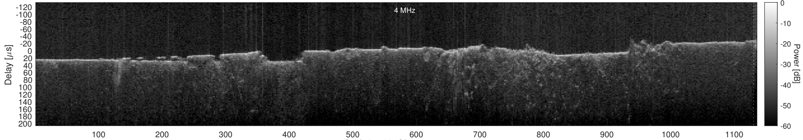
Orbit 21700, Cluttergram
