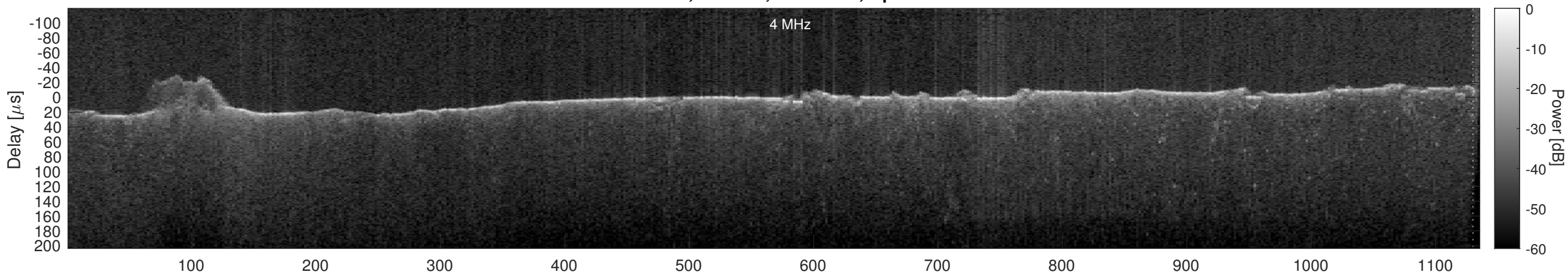
Orbit 21701, Cluttergram
