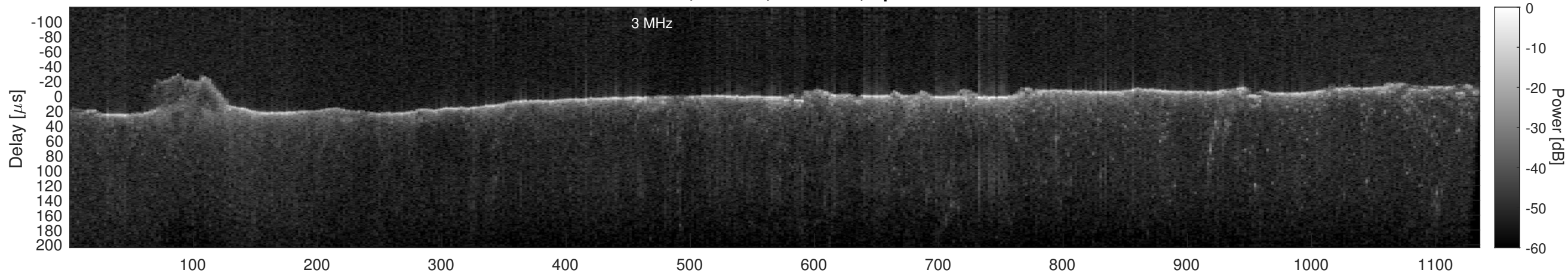
Orbit 21701, Cluttergram
