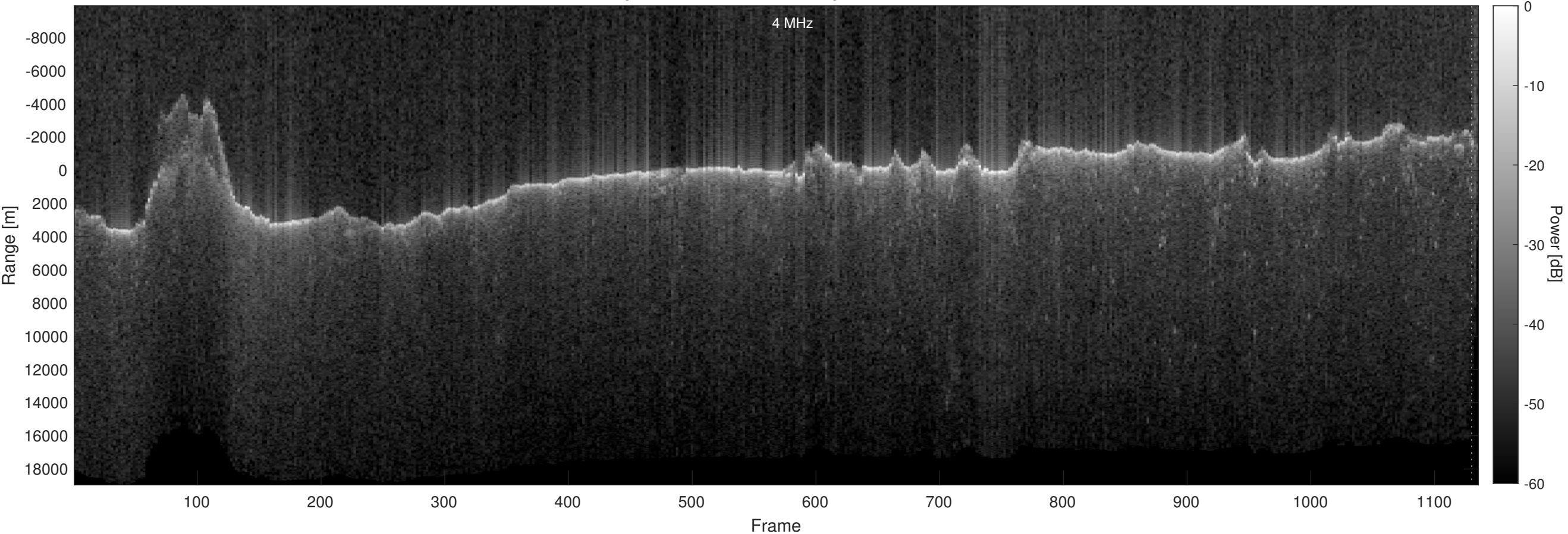
Orbit 21701, Optimized, No Window, Depth-Corrected, Channel 2
