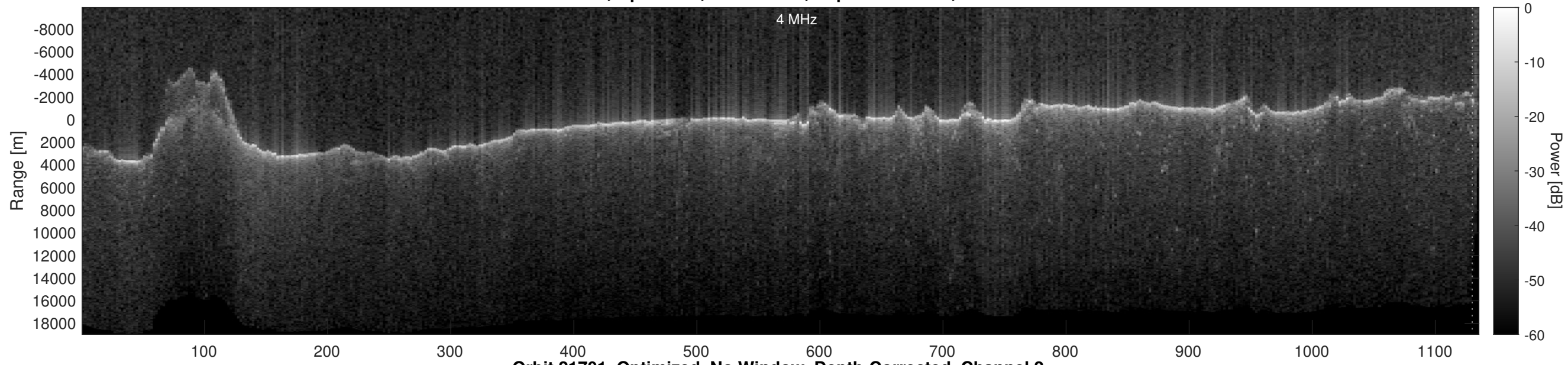
Orbit 21701, Optimized, No Window, Depth-Corrected, Channel 2
