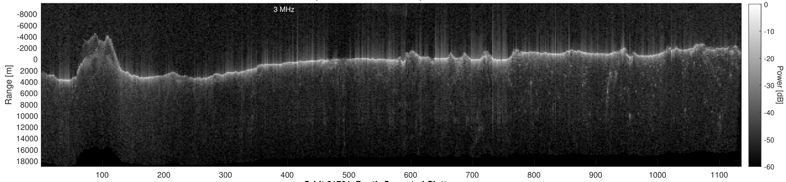
Orbit 21701, Depth-Corrected Cluttergram
