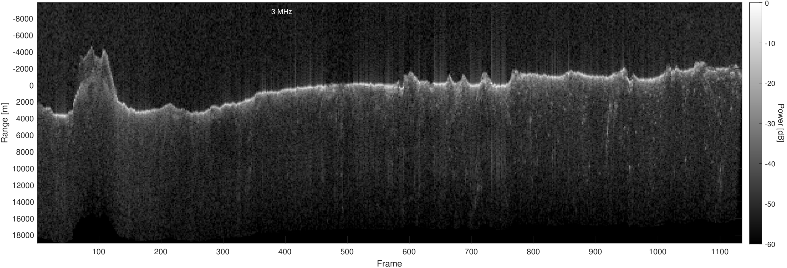
Orbit 21701, Optimized, Window, Depth-Corrected, Channel 2
