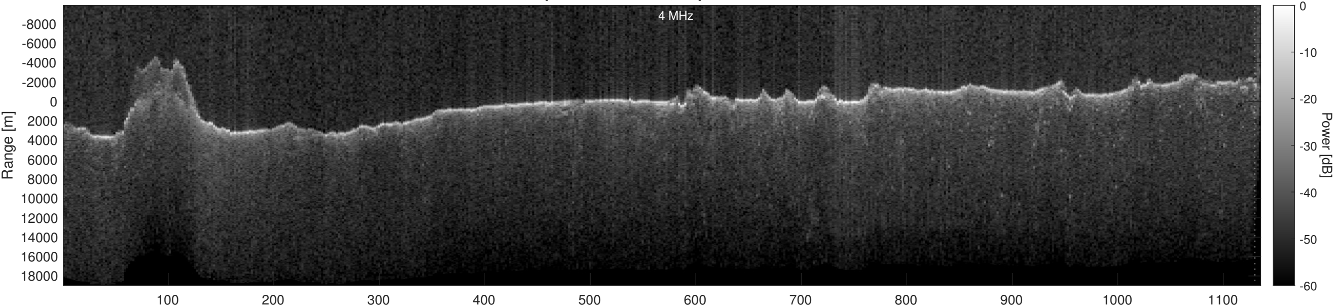
Orbit 21701, Optimized, Window, Depth-Corrected, Channel 2
