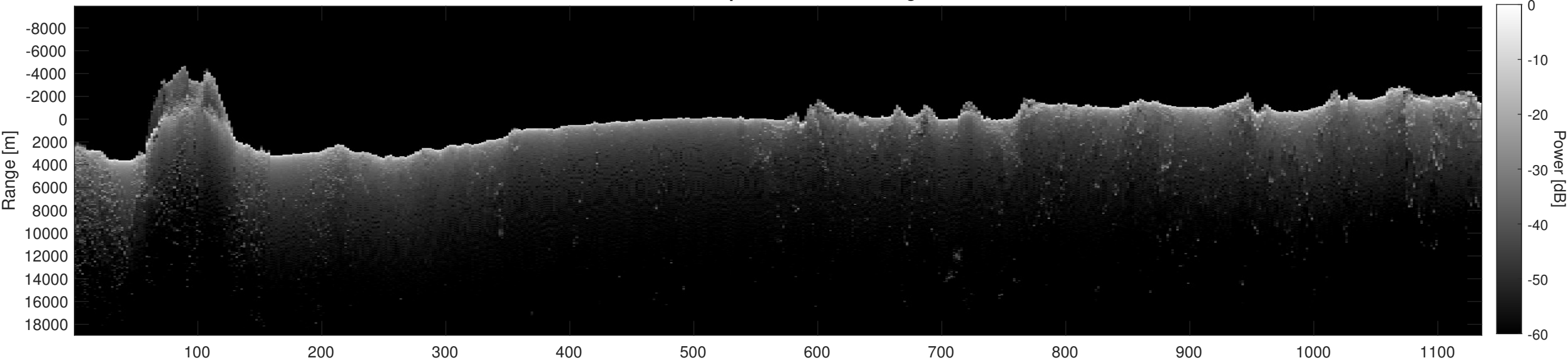
Orbit 21701, Depth-Corrected Cluttergram
