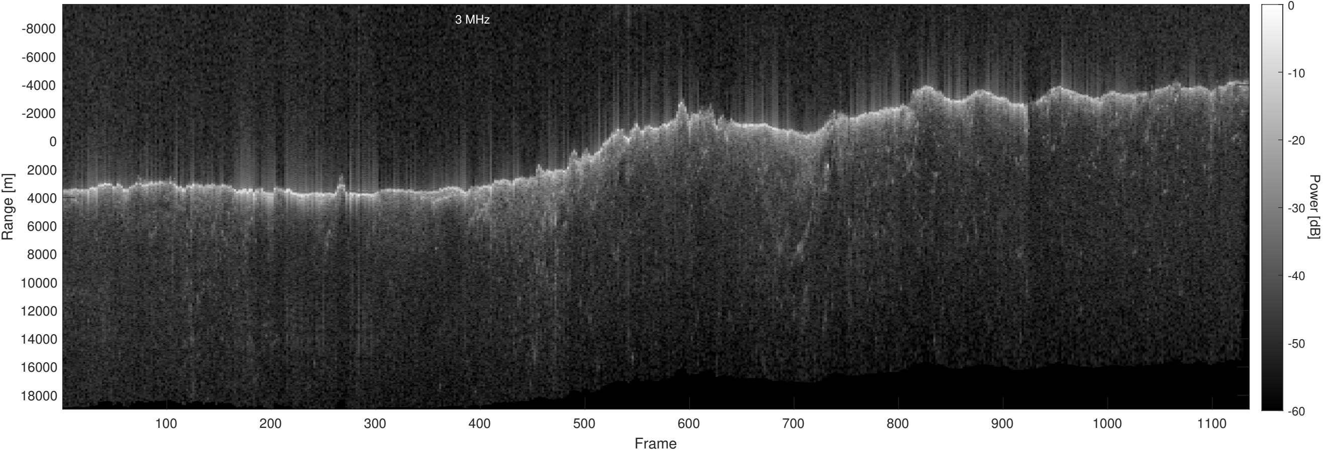
Orbit 21705, Optimized, No Window, Depth-Corrected, Channel 2
