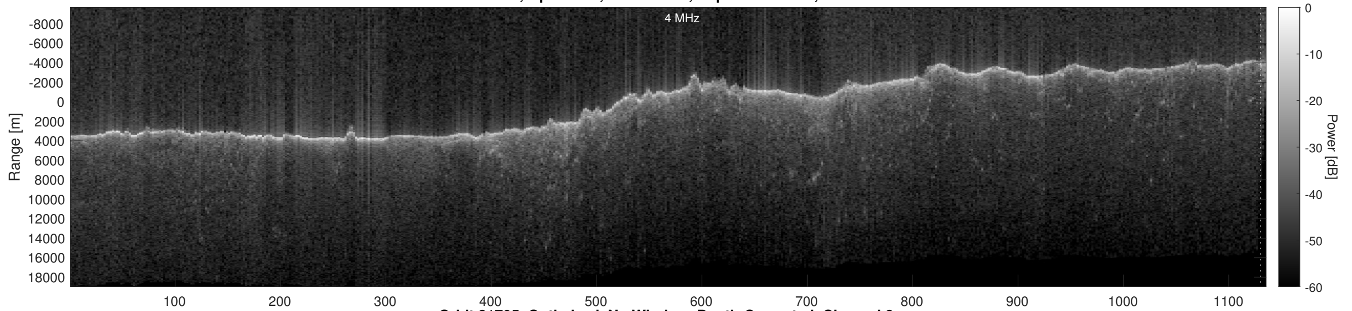
Orbit 21705, Optimized, No Window, Depth-Corrected, Channel 2
