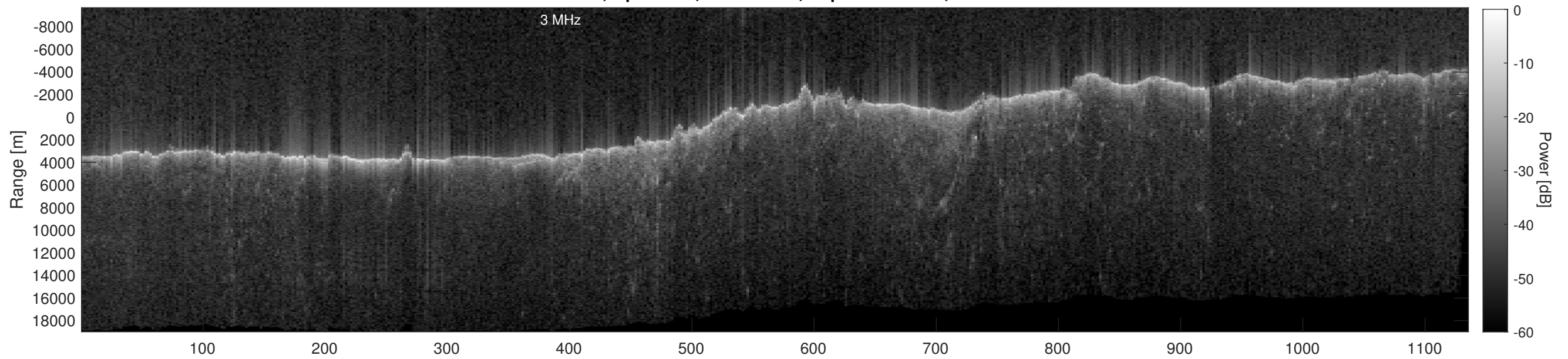
Orbit 21705, Depth-Corrected Cluttergram
