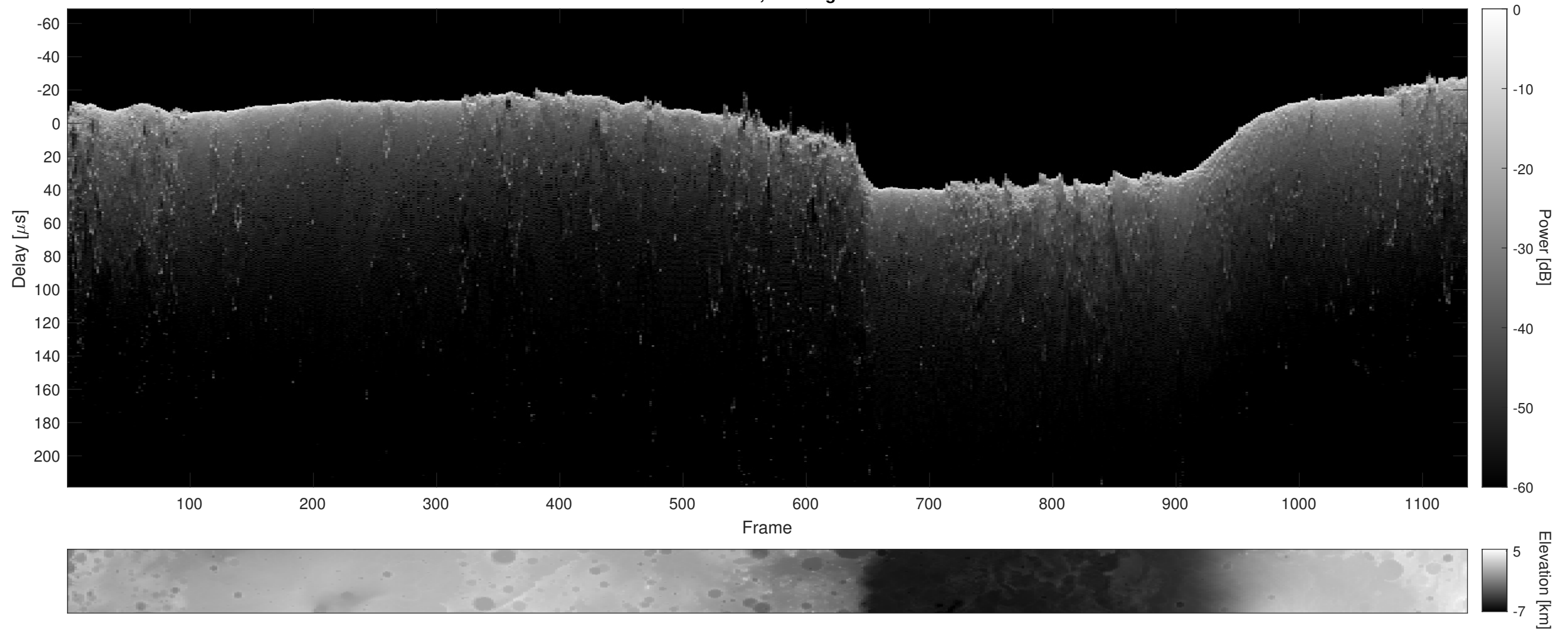
Orbit 21706, Cluttergram
