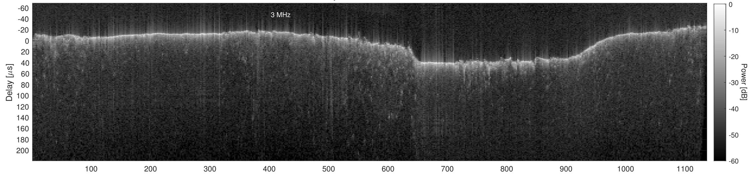
Orbit 21706, Cluttergram
