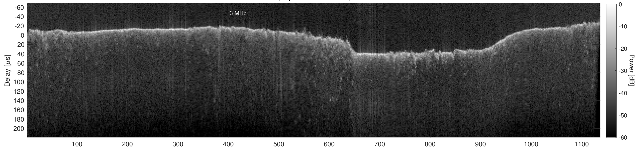
Orbit 21706, Cluttergram
