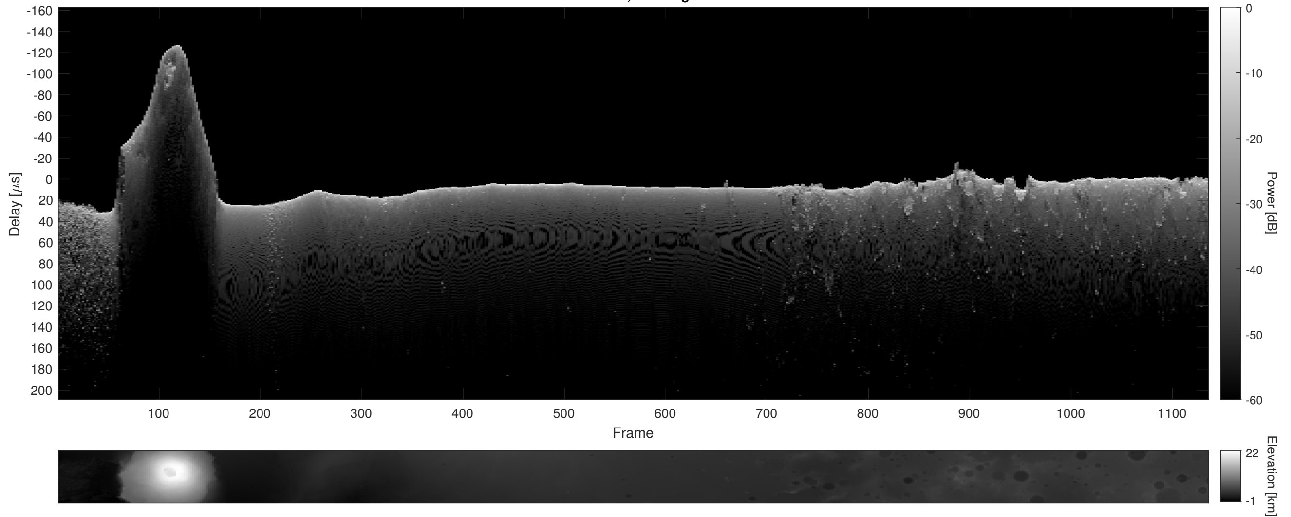
Orbit 21708, Cluttergram
