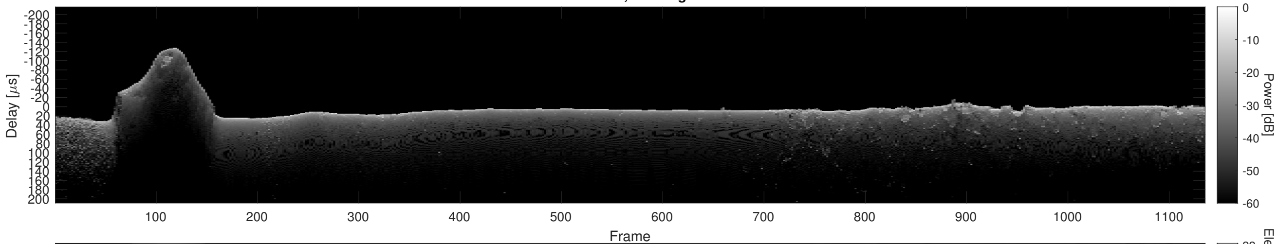
Orbit 21708, Cluttergram
