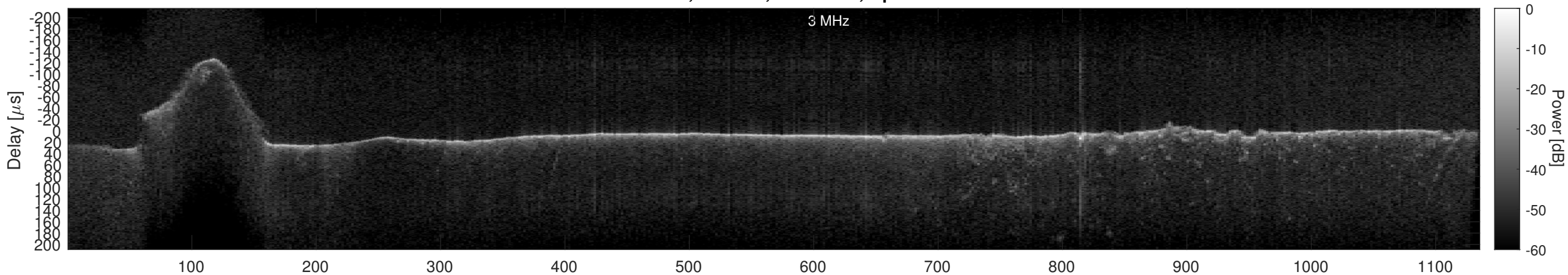
Orbit 21708, Cluttergram
