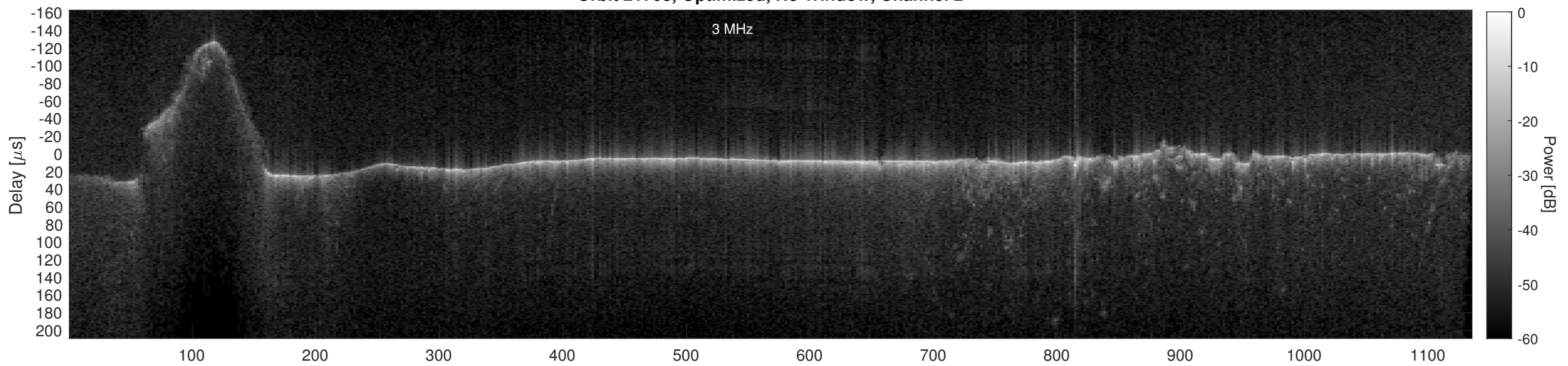
Orbit 21708, Cluttergram
