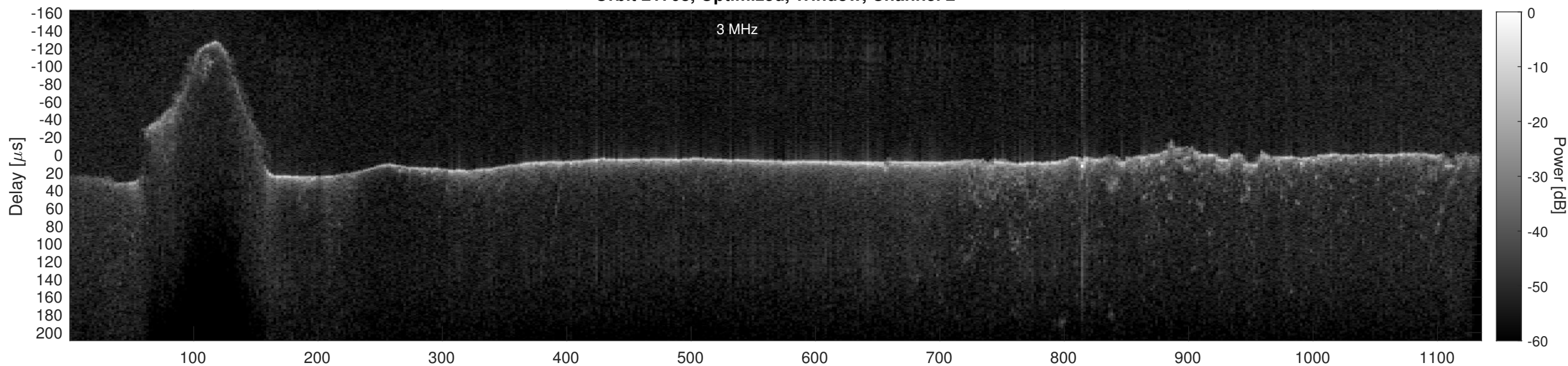
Orbit 21708, Cluttergram
