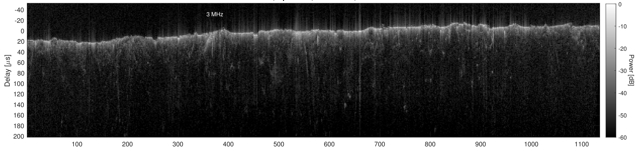
Orbit 21710, Cluttergram
