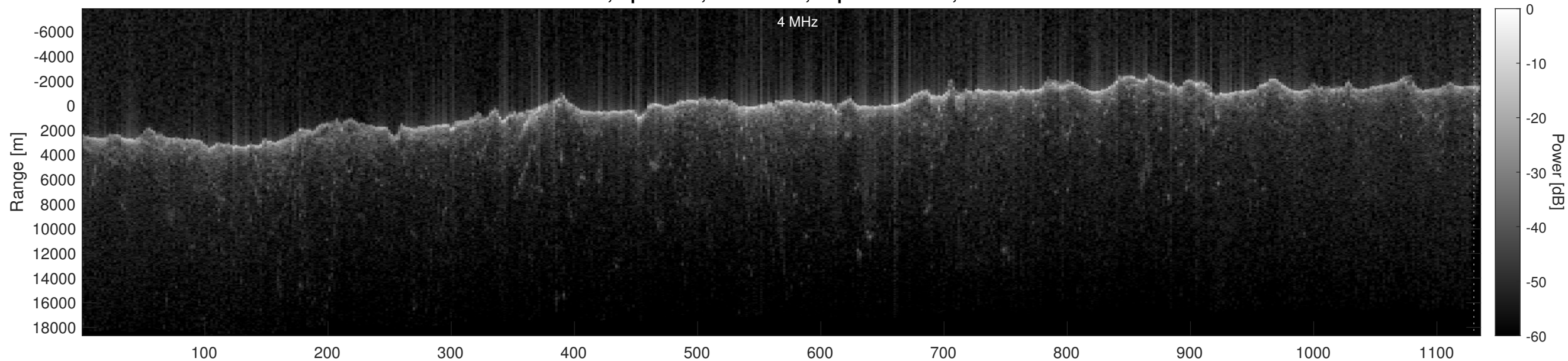
Orbit 21710, Optimized, No Window, Depth-Corrected, Channel 2
