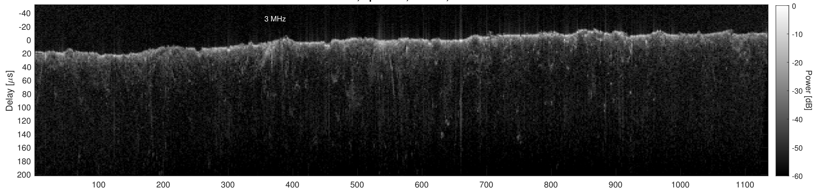
Orbit 21710, Cluttergram
