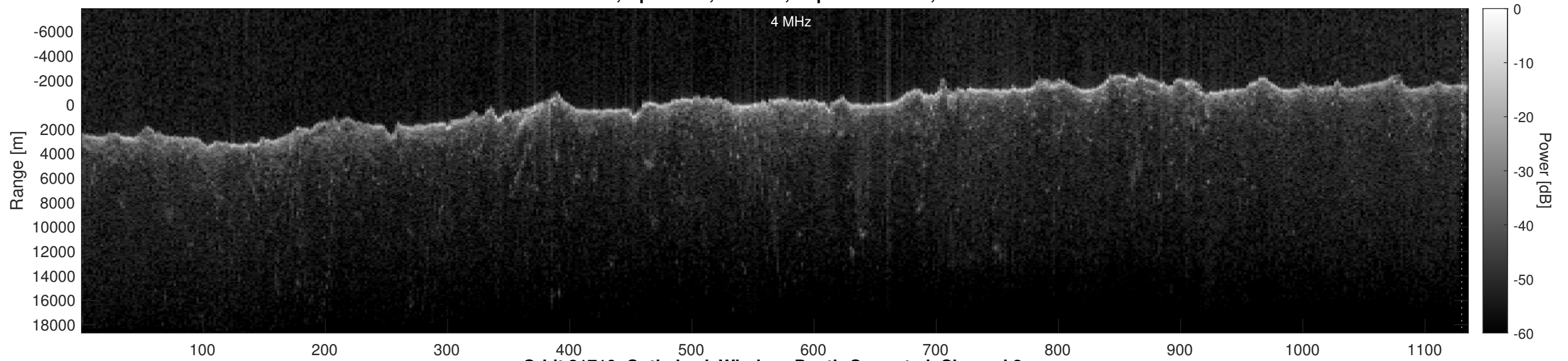
Orbit 21710, Optimized, Window, Depth-Corrected, Channel 2
