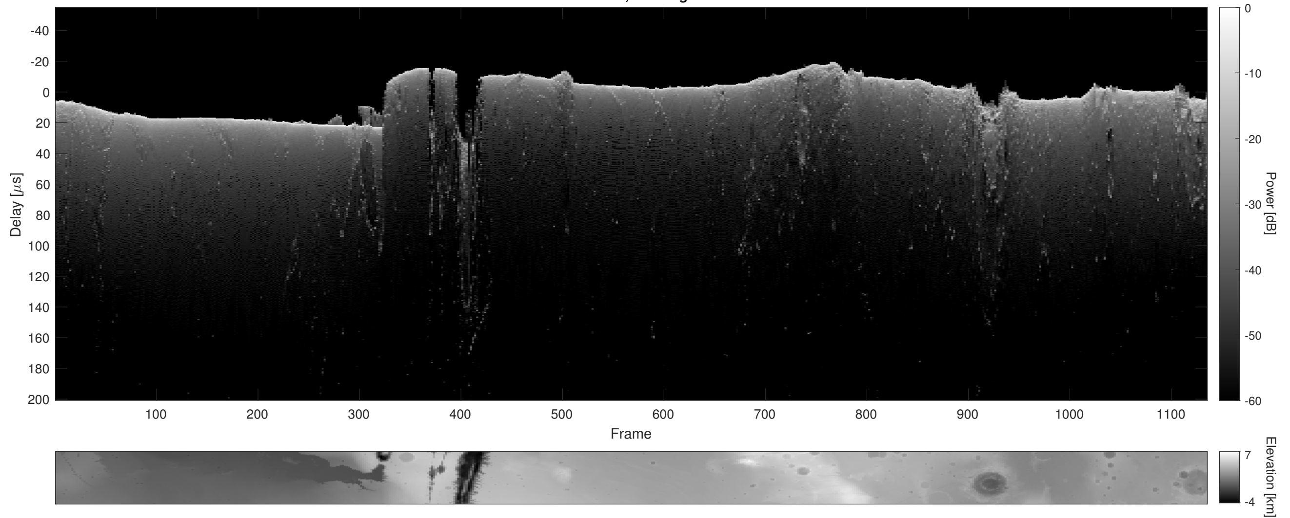
Orbit 21711, Cluttergram
