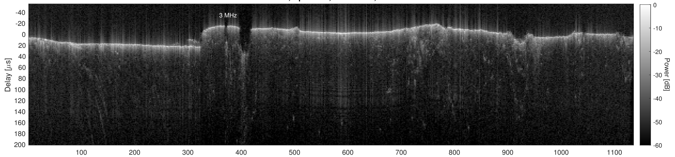
Orbit 21711, Cluttergram
