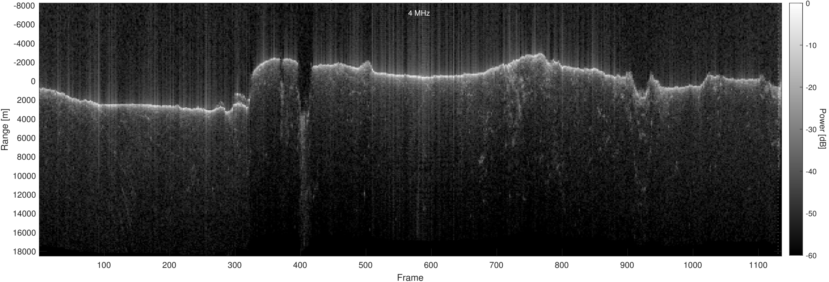
Orbit 21711, Optimized, No Window, Depth-Corrected, Channel 2
