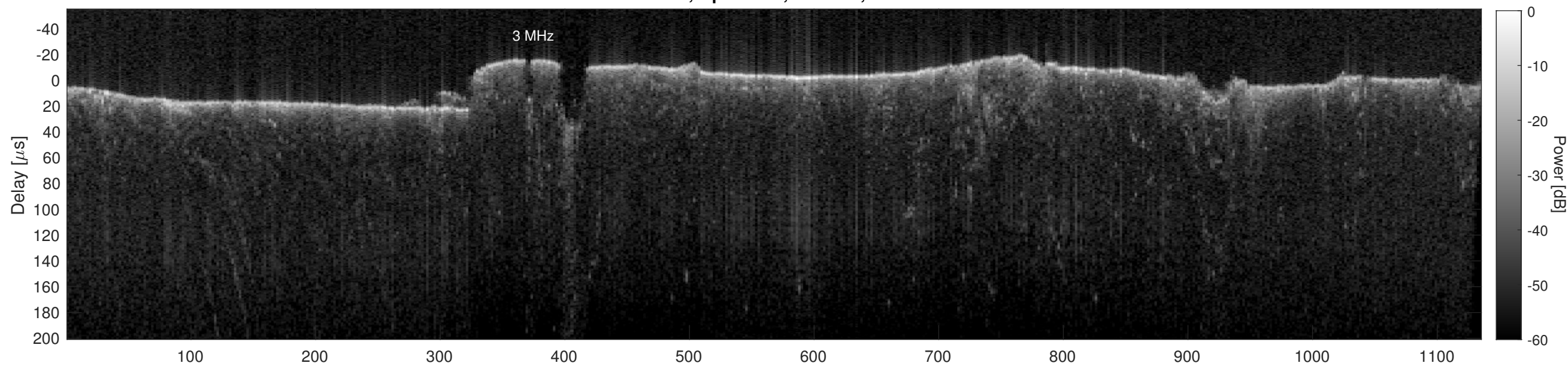
Orbit 21711, Cluttergram
