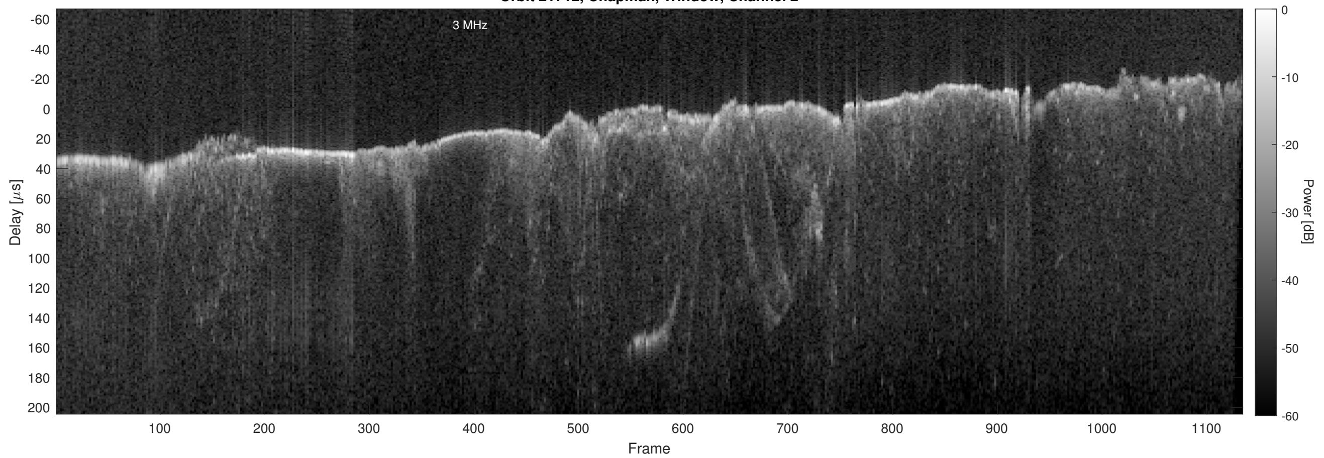
Orbit 21712, Chapman, Window, Channel 2
