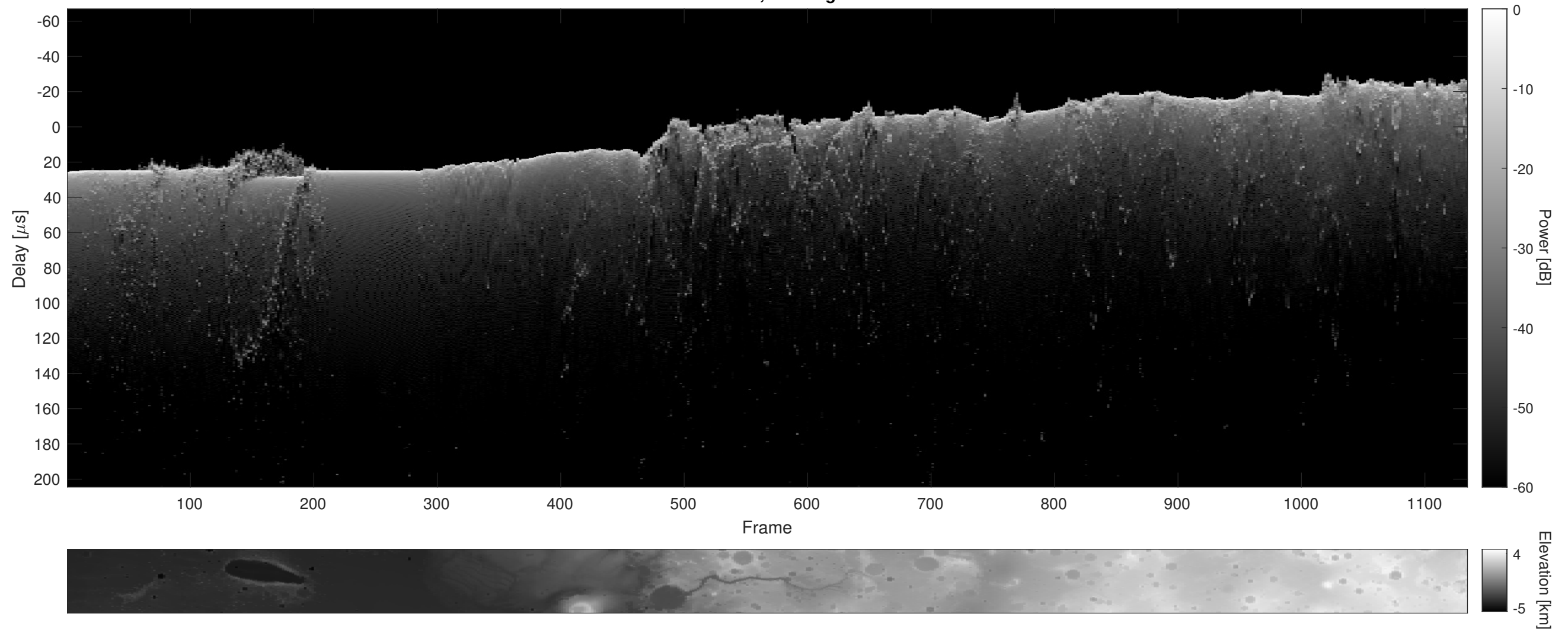
Orbit 21712, Cluttergram
