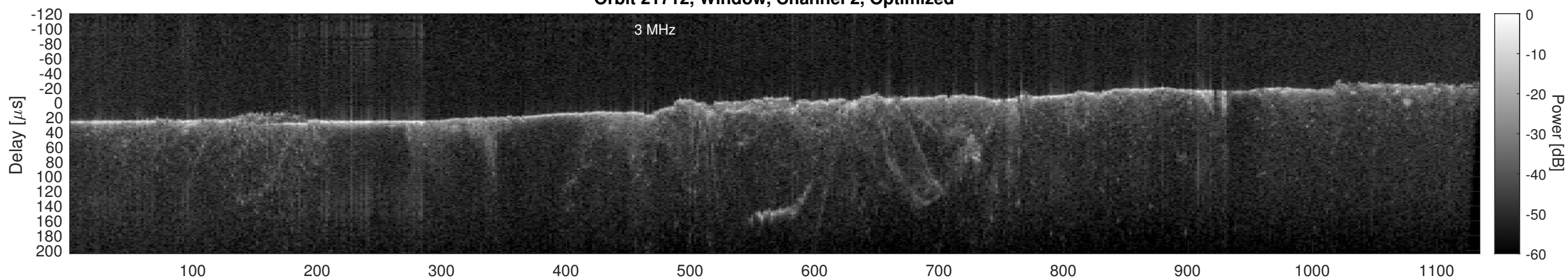
Orbit 21712, Cluttergram
