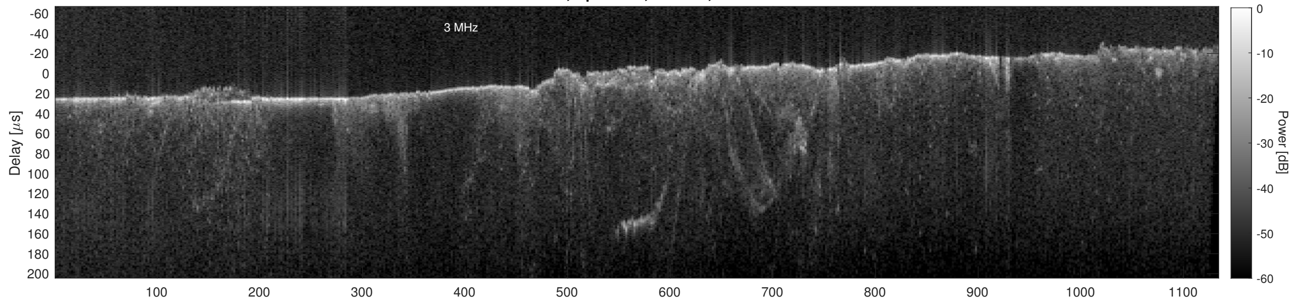
Orbit 21712, Cluttergram
