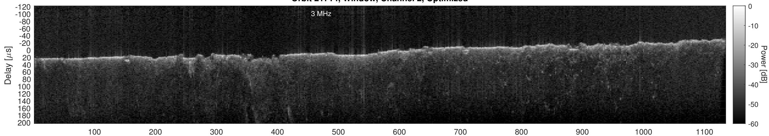
Orbit 21714, Cluttergram
