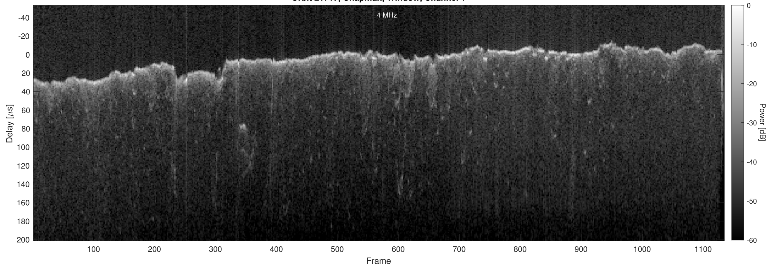
Orbit 21717, Chapman, Window, Channel 2
