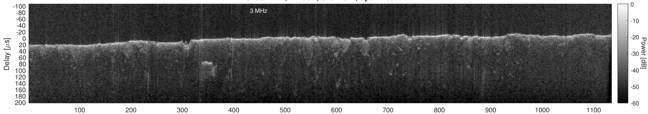
Orbit 21717, Cluttergram
