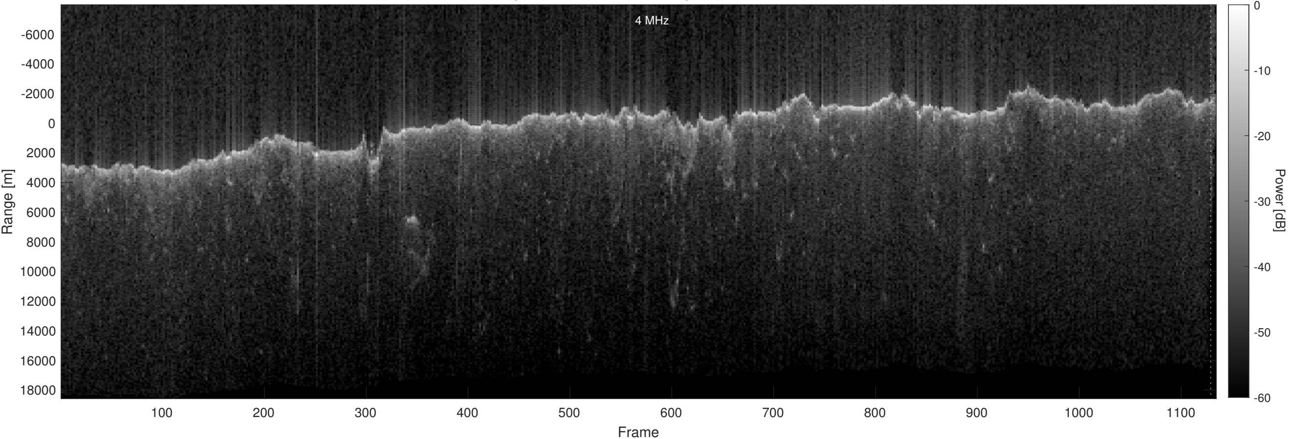
Orbit 21717, Optimized, No Window, Depth-Corrected, Channel 2
