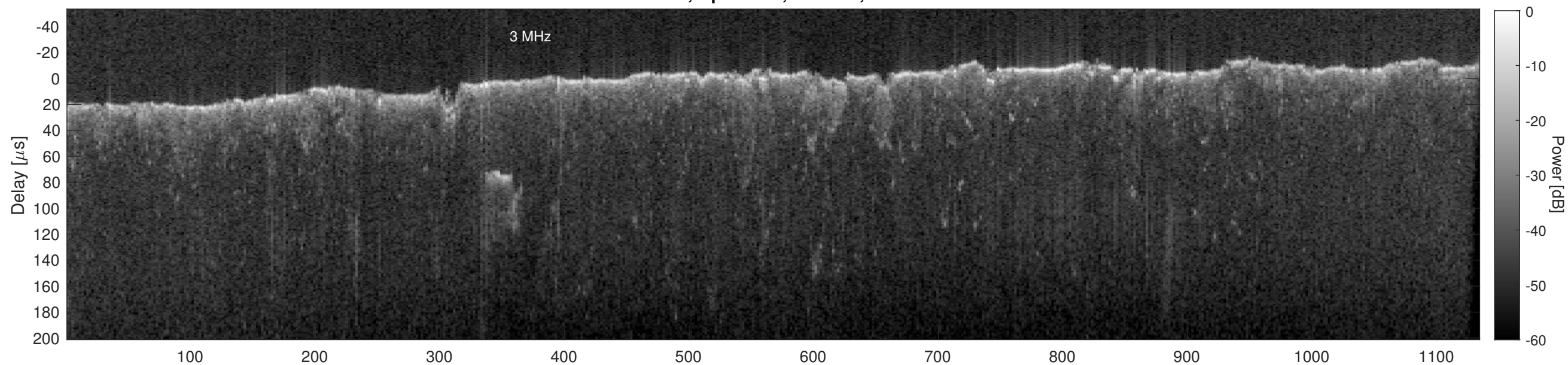
Orbit 21717, Cluttergram
