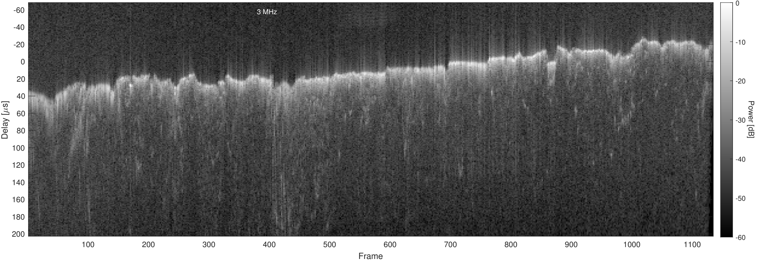
Orbit 21721, Chapman, No Window, Channel 2
