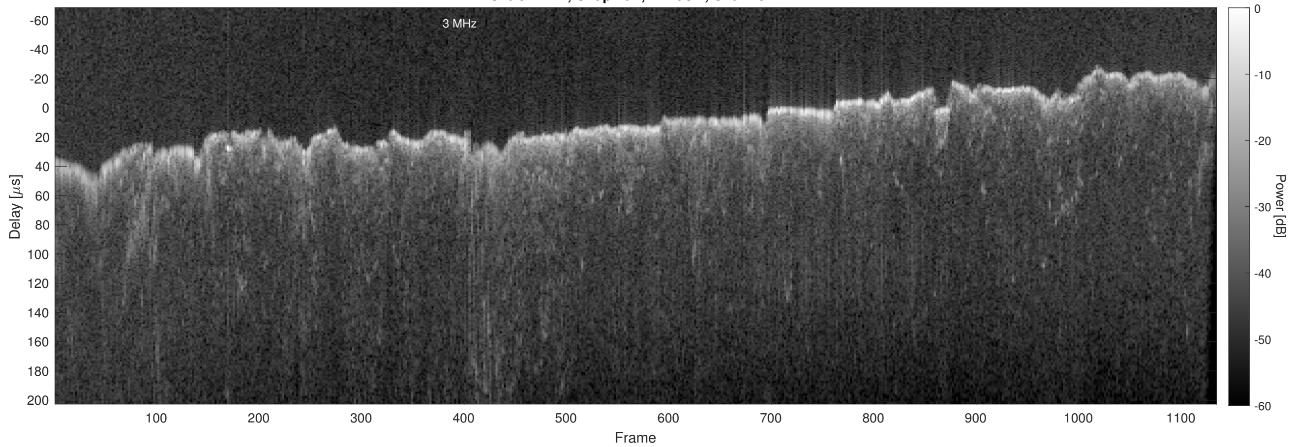
Orbit 21721, Chapman, Window, Channel 2
