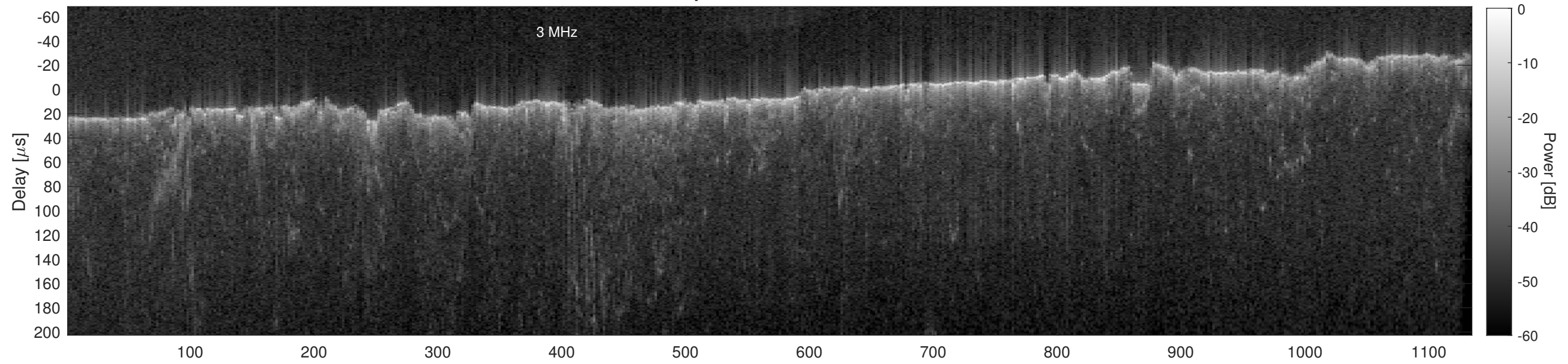
Orbit 21721, Cluttergram
