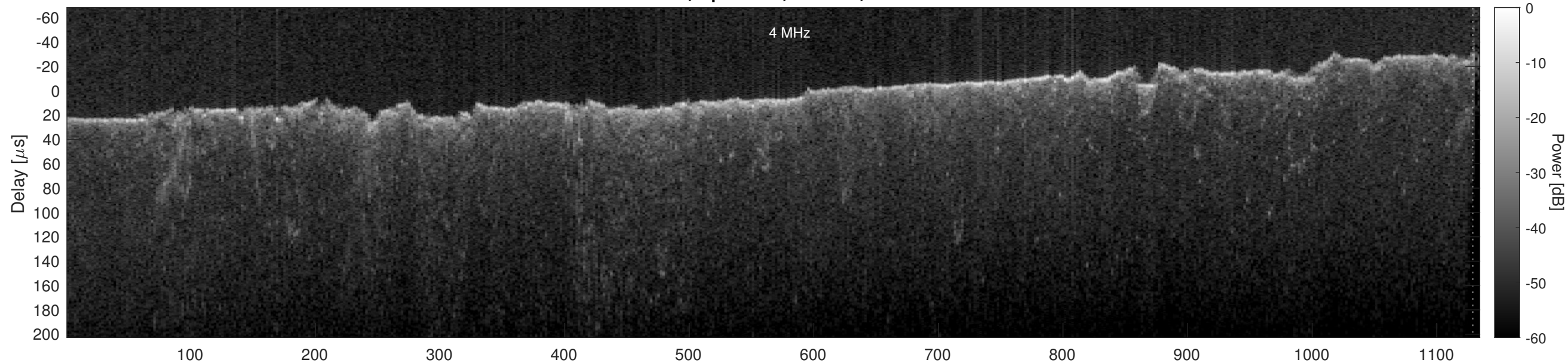
Orbit 21721, Optimized, Window, Channel 2
