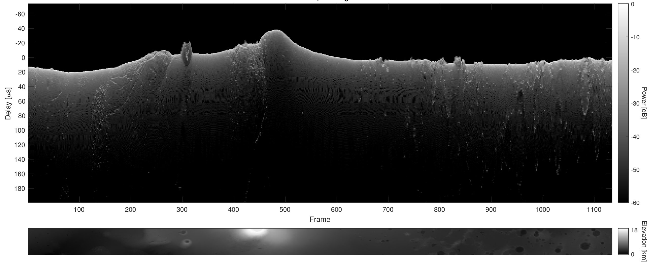
Orbit 21722, Cluttergram
