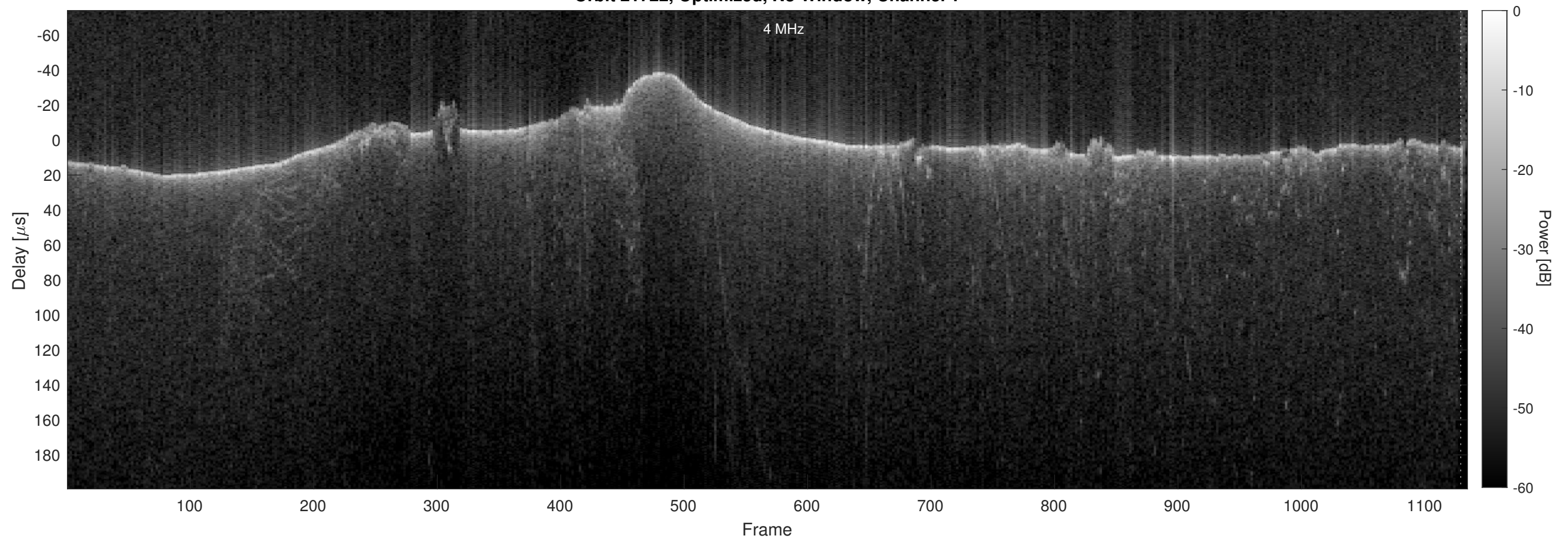
Orbit 21722, Optimized, No Window, Channel 2
