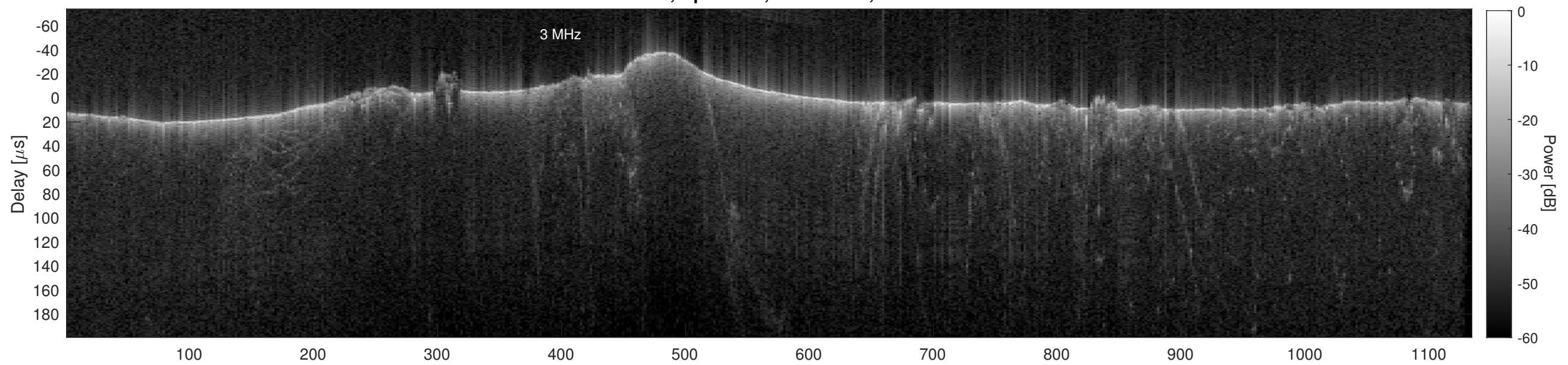
Orbit 21722, Cluttergram
