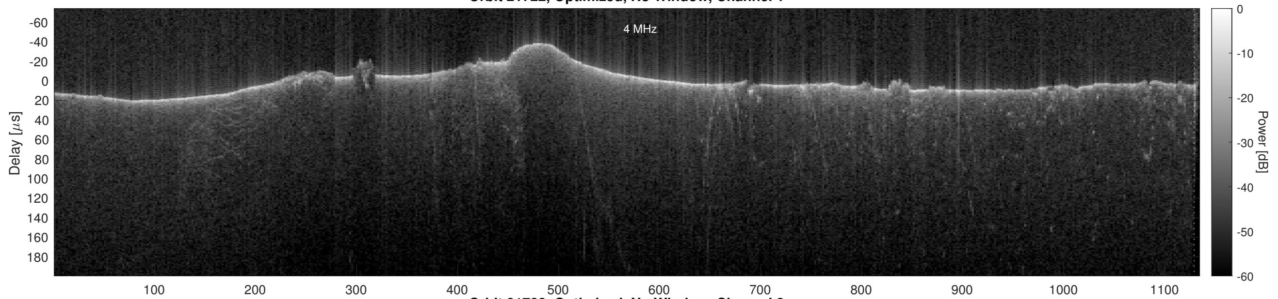
Orbit 21722, Optimized, No Window, Channel 2
