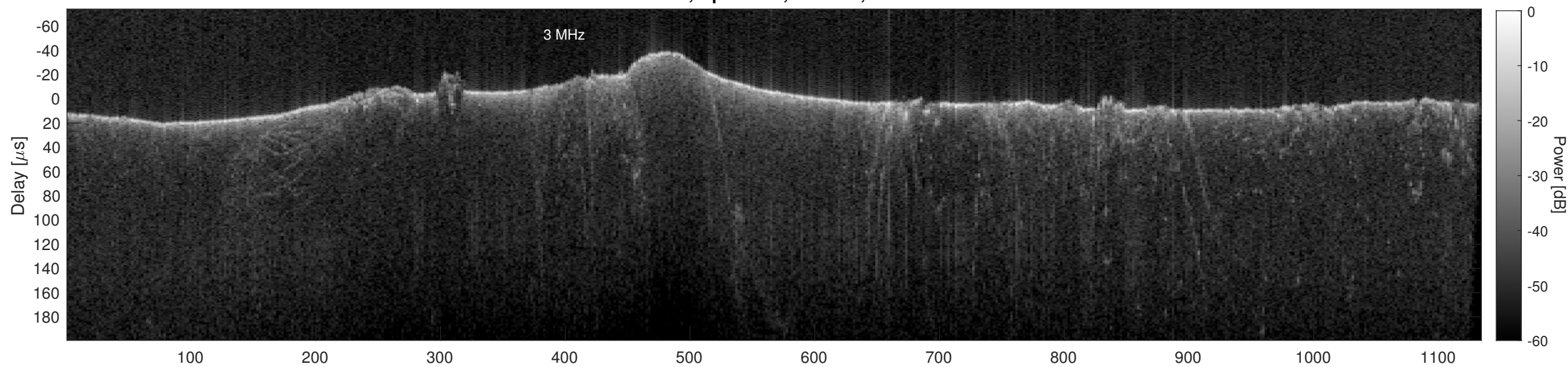
Orbit 21722, Cluttergram
