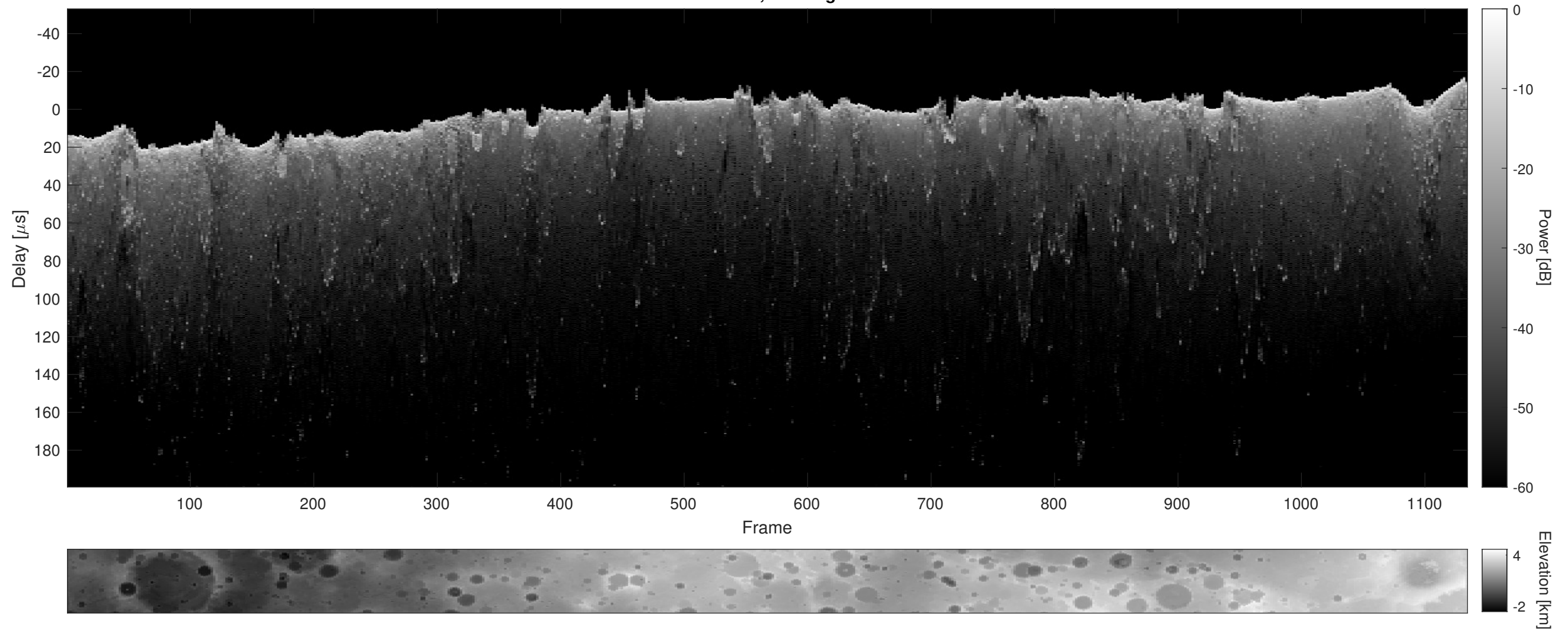
Orbit 21724, Cluttergram
