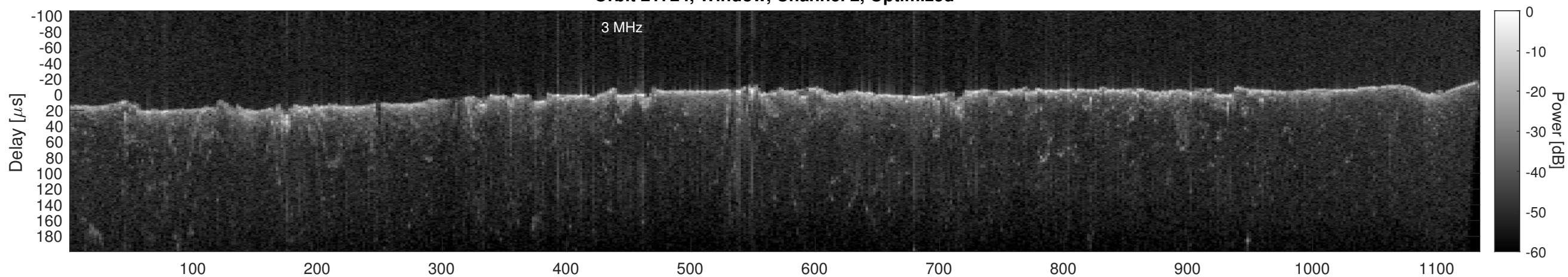
Orbit 21724, Cluttergram
